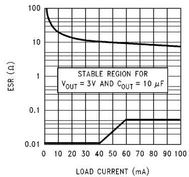
FIGURE 4. 3V/10 \mu F ESR Curves
