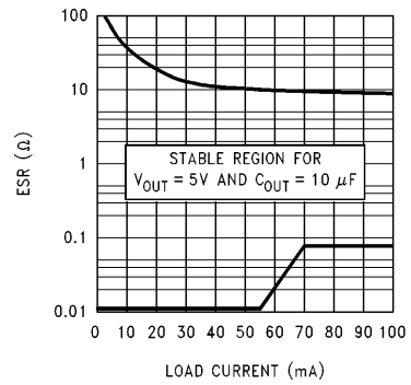
FIGURE 2. 5V/10 \mu F ESR Curves
