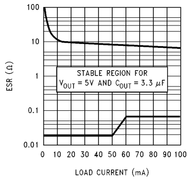
FIGURE 1. 5V/3.3 \mu F ESR Curves
