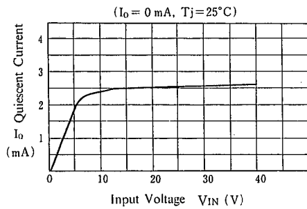
NJM78L05 Quiescent Current vs. Input Voltage ( I_o = 0 mA, T_j = 25^\circ\text{C} )
